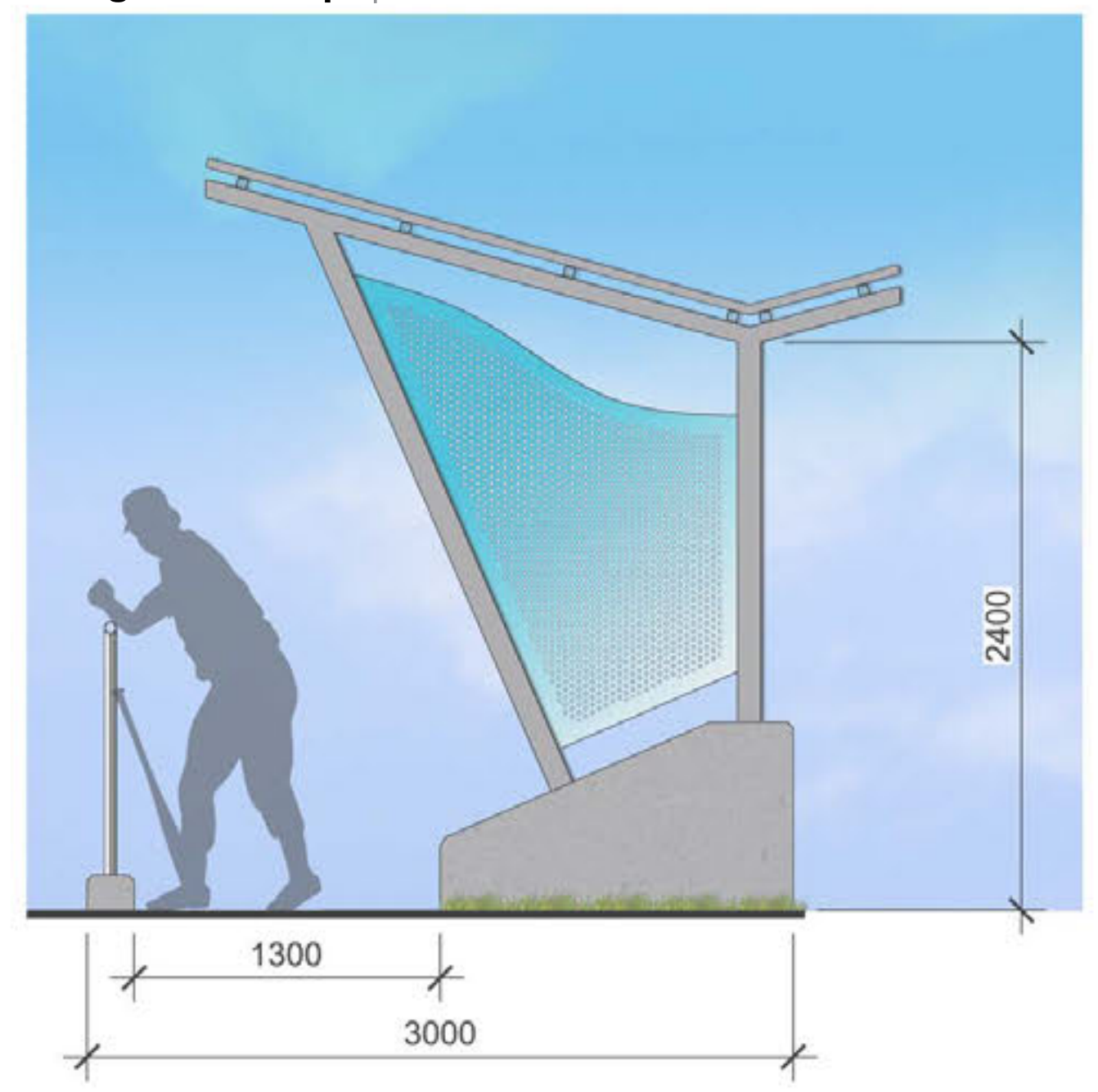
Dugout Concept | Side Elevation
